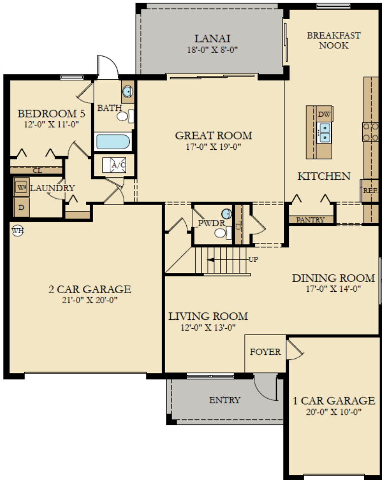
FIRST FLOOR
